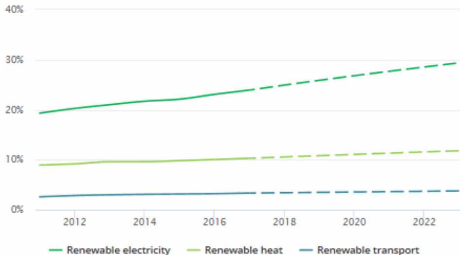
Share of modern renewable energy by sector, 2011-23
